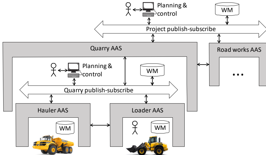
Fig. 3. Hierarchical decomposition of a road construction SoS.
