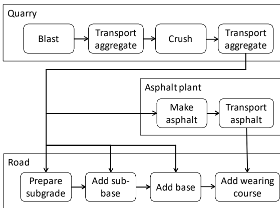
Fig. 1. Overview of road construction processes.
